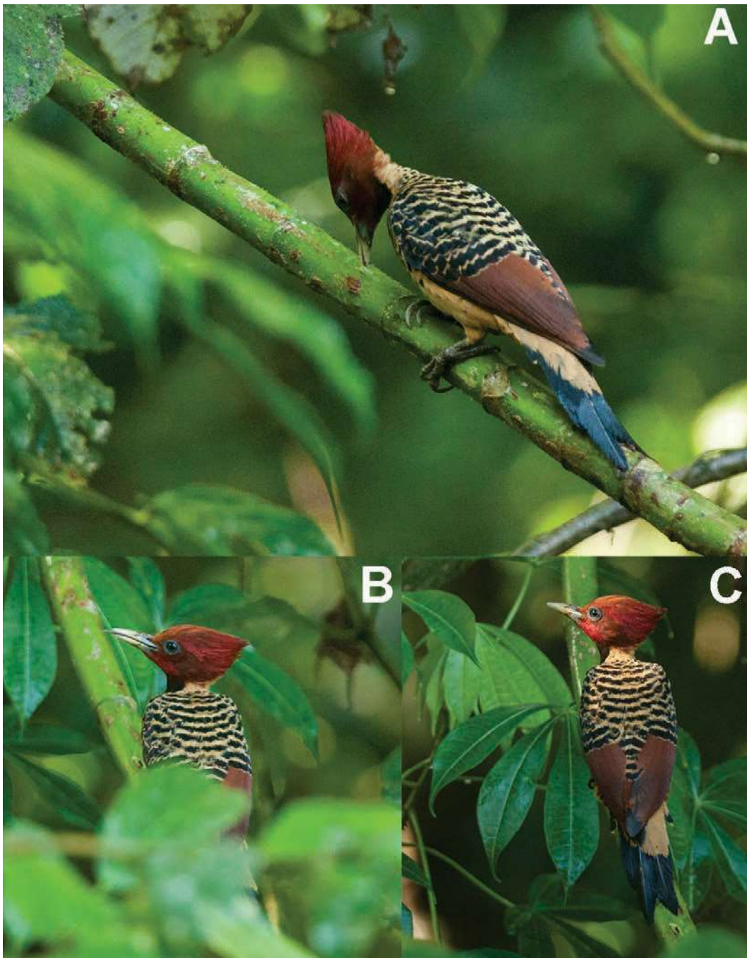
Figure 2. Rufous-headed Woodpecker Celeus spectabilis foraging in a Cecropia tree: (A) pecking a hole when first spotted at 15h00; (B) after eating an ant; (C) and a few seconds before departing from the Cecropia tree (Giselle Mangini & Oliver Thomas)
